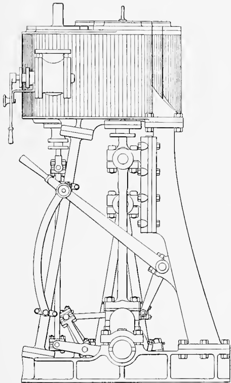
TRIPLE-EXPANSION ENGINE OF ISAAC BEARINGER'S STEAM YACHT WAPITI.
